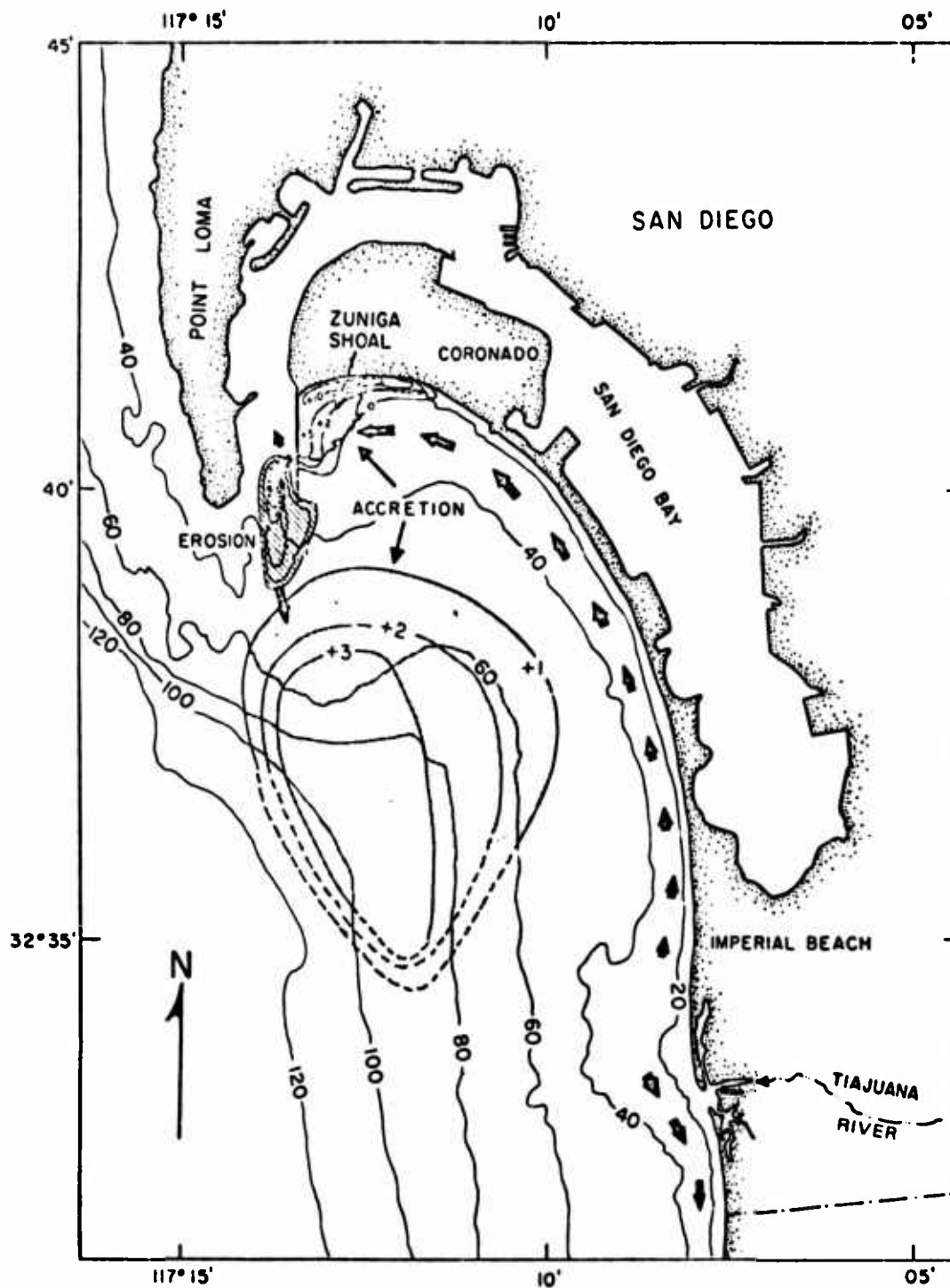
Figure 10. Silver Strand littoral cell, showing the Tiajuana river as the former source of natural sand, the littoral transport paths north along the Silver Strand, and the deposition areas; the final deposition area is the offshore region indicated by the isolines determined by comparing surveys of 1923 and 1934. (Source: Inmann, 1973.)
